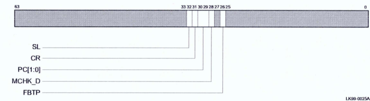
Figure 5–19 Hardware Interrupt Clear Register
