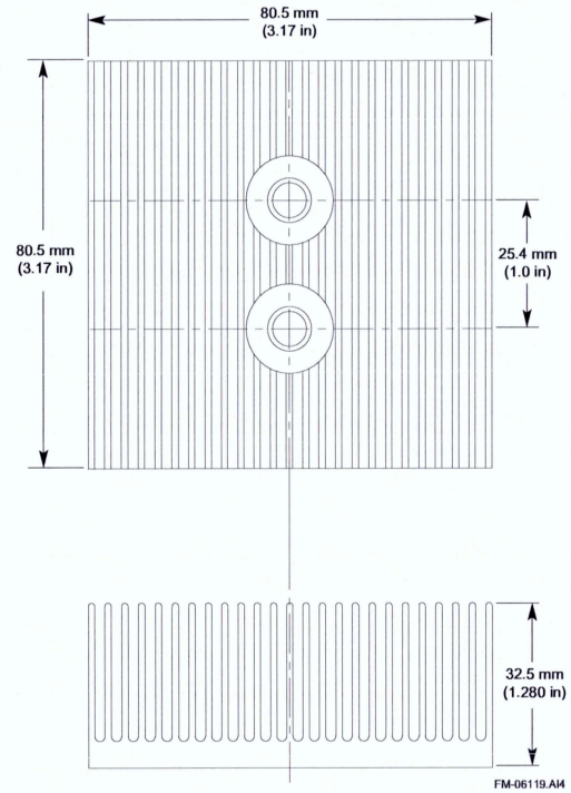
Figure 10-1 Type 1 Heat Sink
