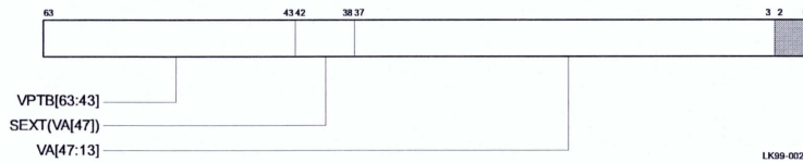
Figure 5–14 Instruction Virtual Address Format Register (VA_48 = 1, VA_FORM_32 = 0)
