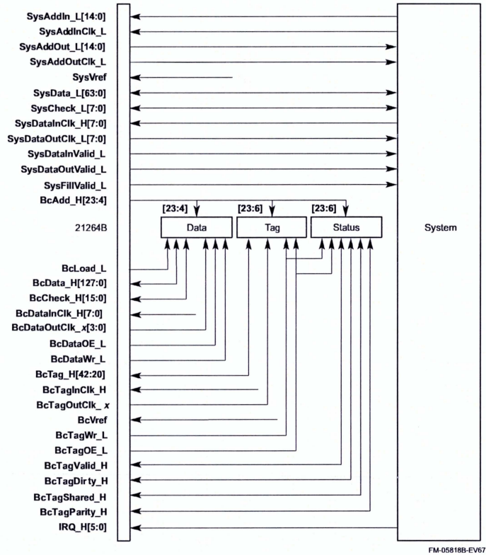
Figure 4–1 21264B System and Bcache Interfaces
