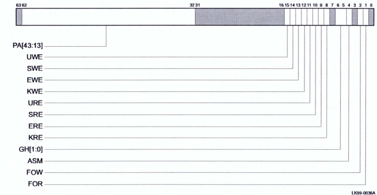
Figure 5–27 DTB PTE Array Write Registers 0 and 1
