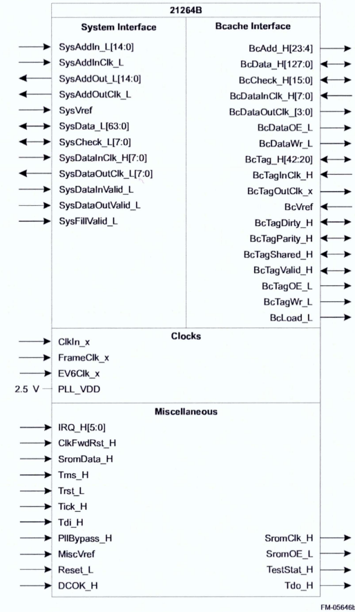
Figure 3–1 21264B Microprocessor Logic Symbol
