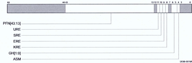
Figure 5–9 ITB PTE Array Write Register
