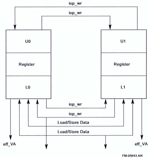
Figure 2-6 Integer Execution Unit—Clusters 0 and 1
