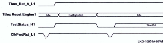
Figure 11–2 TestStat_H Pin Timing During Built-In Self-Initialization (BiSI)
