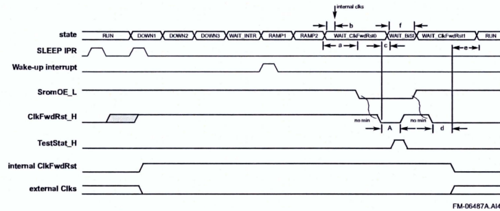
Figure 7–3 Sleep Mode Sequence of Operation
