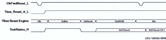
Figure 11–1 TestStat_H Pin Timing During Power-Up Built-In Self-Test (BiST)
