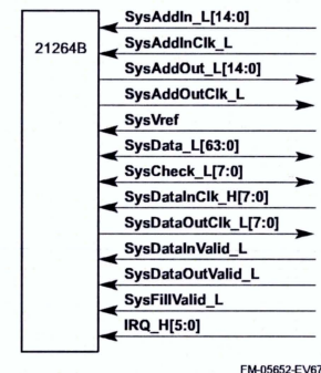
Figure 4–4 System Interface Signals
