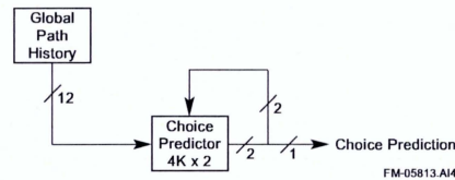
Figure 2-5 Choice Predictor
