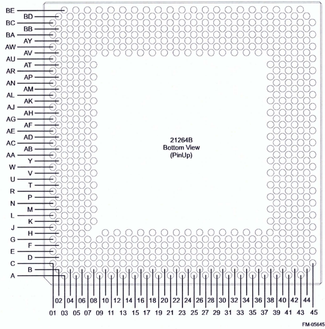
Figure 3-4 21264B Bottom View (Pin Up)
