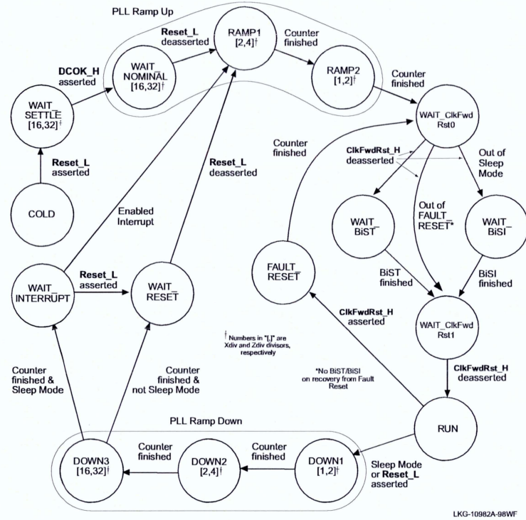
Figure 7–5 21264B Reset State Machine State Diagram
