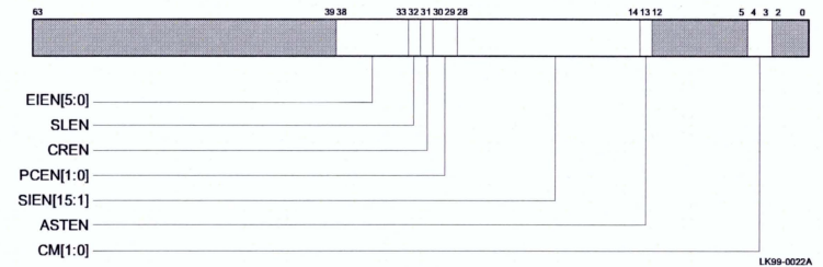
Figure 5–16 Interrupt Enable and Current Processor Mode Register
