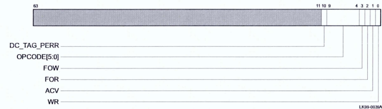
Figure 5–31 Memory Management Status Register
