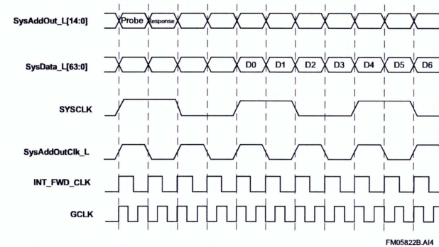
Figure 4–5 Fast Transfer Timing Example
