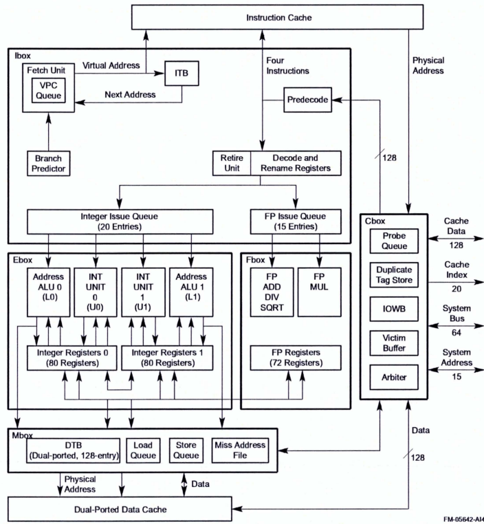
Figure 2-1 21264B Block Diagram
