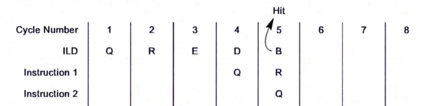
Figure 2–9 Pipeline Timing for Integer Load Instructions
