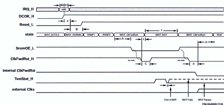
Figure 7–1 Power-Up Timing Sequence
