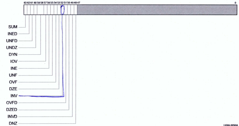
Figure 2–11 Floating-Point Control Register
