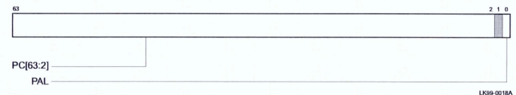
Figure 5–12 Exception Address Register
