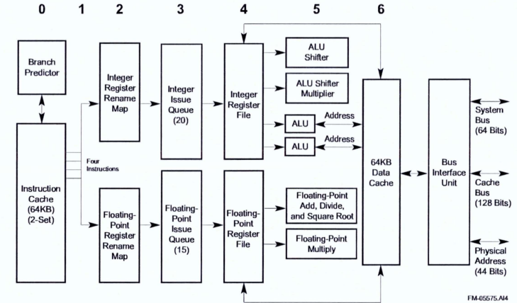
Figure 2-8 Pipeline Organization
