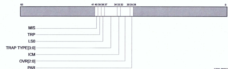
Figure 5–23 Ibox Status Register
