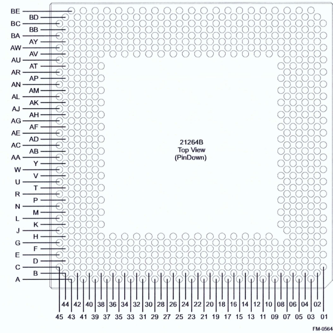
Figure 3–3 21264B Top View (Pin Down)
