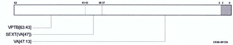
Figure 5-6 Virtual Address Format Register (VA_48 = 1, VA_FORM_32 = 0)
