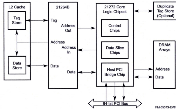
Figure 2-12 Typical Uniprocessor Configuration
