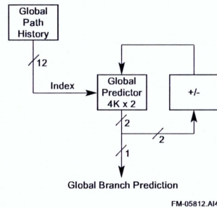
Figure 2-4 Global Predictor
