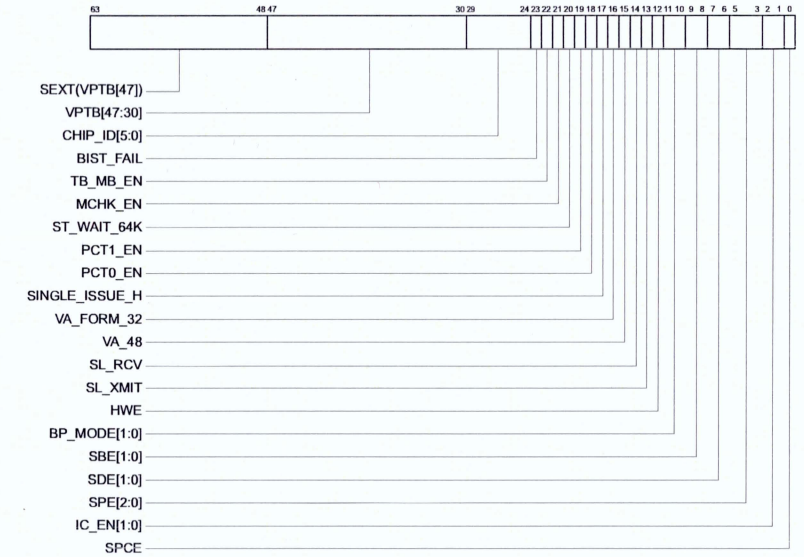
Figure 5–22 Ibox Control Register
