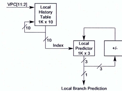
Figure 2-3 Local Predictor
