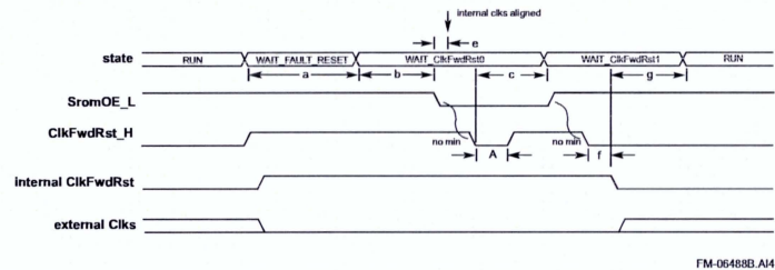
Figure 7–2 Fault Reset Sequence of Operation
