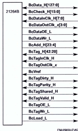
Figure 4–2 21264B Bcache Interface Signals
