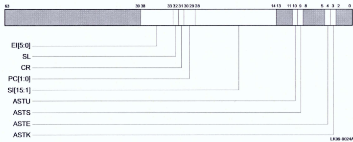
Figure 5–18 Interrupt Summary Register
