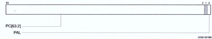
Figure 5–11 ProfileMe PC Register
