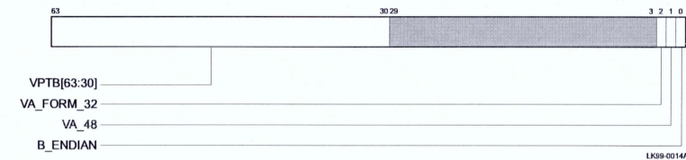
Figure 5-4 Virtual Address Control Register
