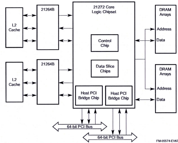
Figure 2-13 Typical Multiprocessor Configuration
