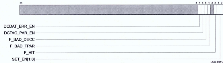
Figure 5–33 Dcache Control Register
