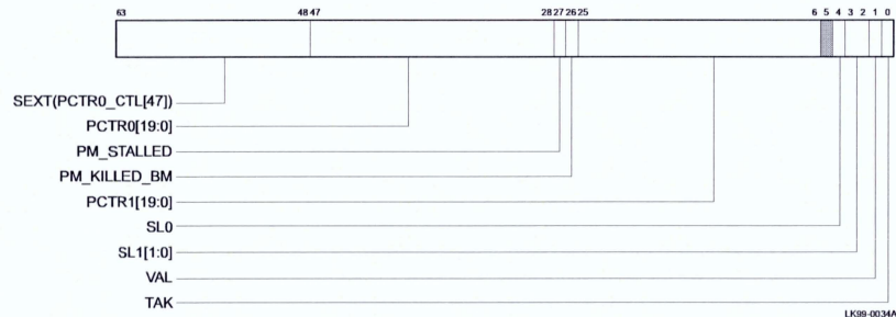
Figure 5–25 Performance Counter Control Register
