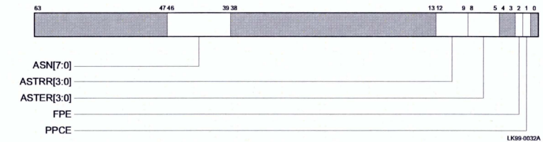
Figure 5–24 Process Context Register
