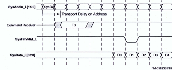
Figure 4–6 SysFillValid_L Timing
