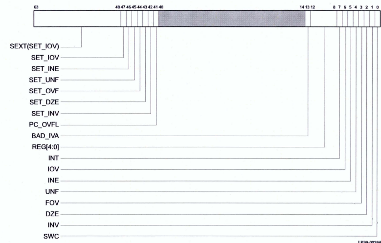
Figure 5–20 Exception Summary Register
