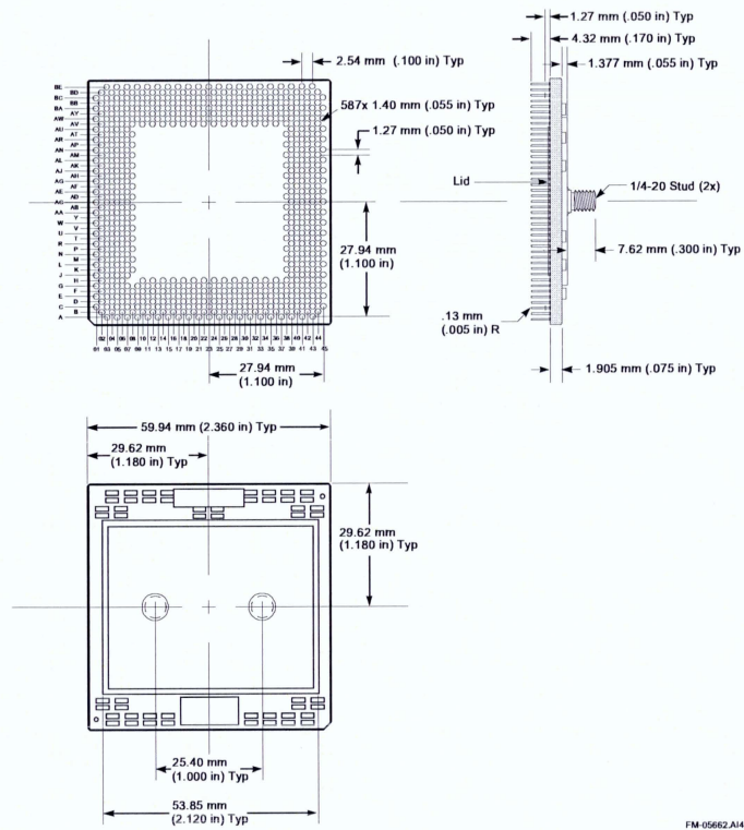
Figure 3–2 Package Dimensions
