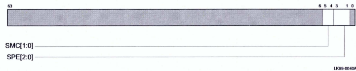
Figure 5–32 Mbox Control Register
